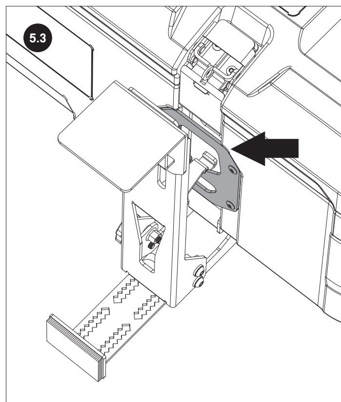
CHECK BOTH REAR HOOKS ARE NOW ENGAGED
